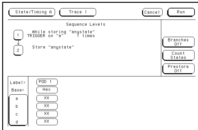
Figure 3-8. Trace Screen
