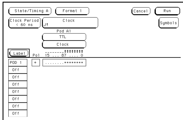
Figure 3-13. Format Screen
