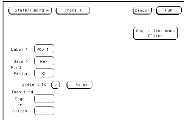
Figure 3-41. Trace Screen
