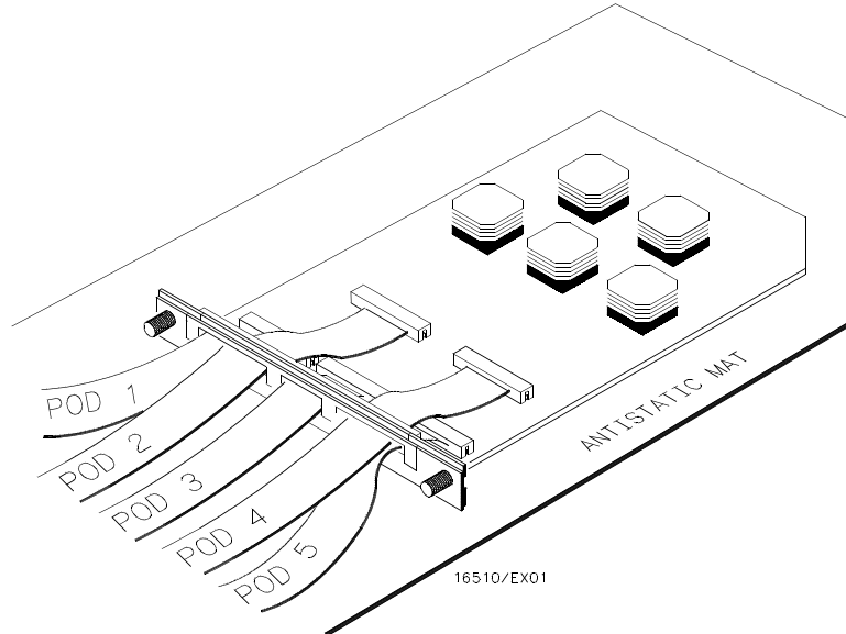
Figure 6-12. Cable Position
