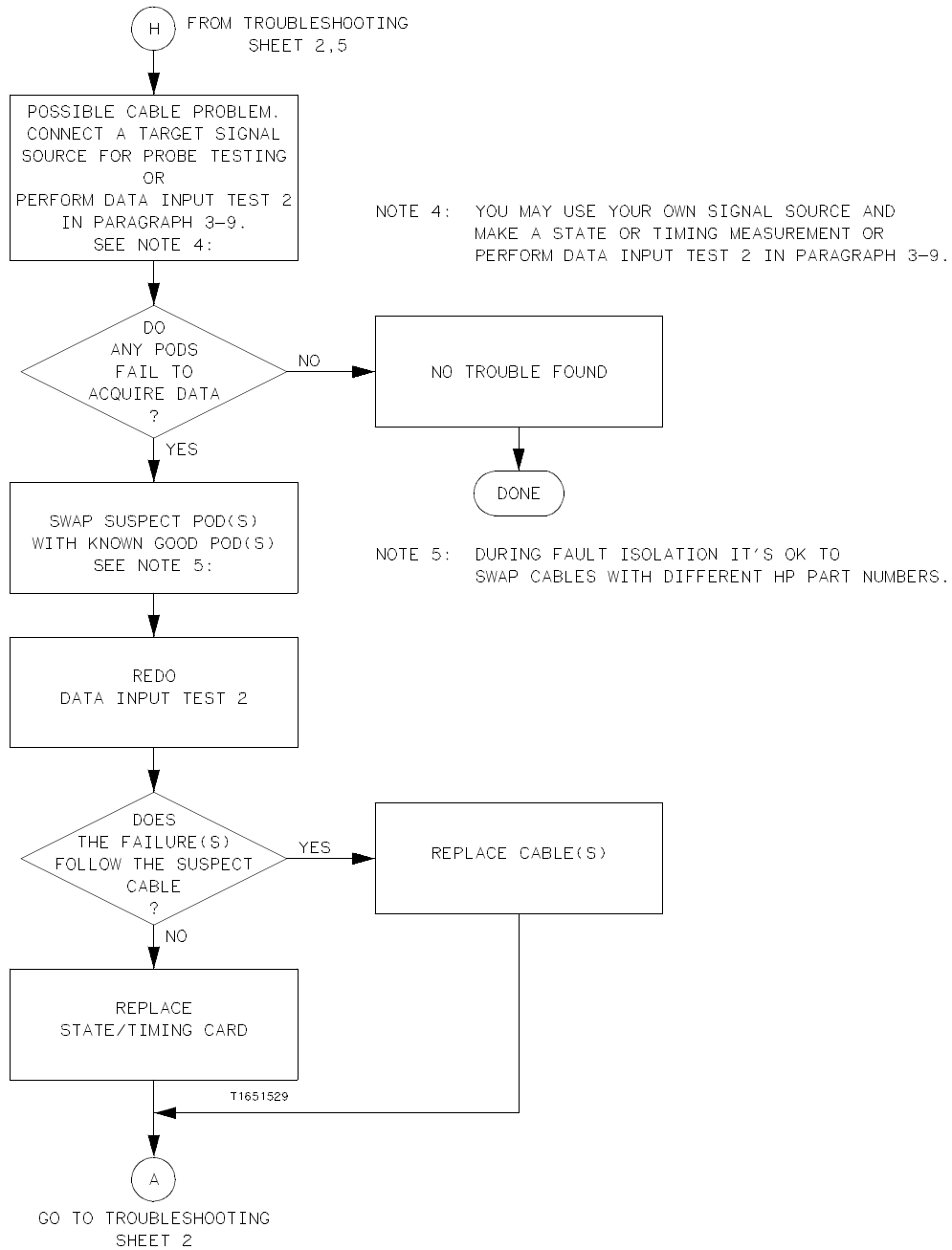
Figure 6-10. Troubleshooting Flowchart
