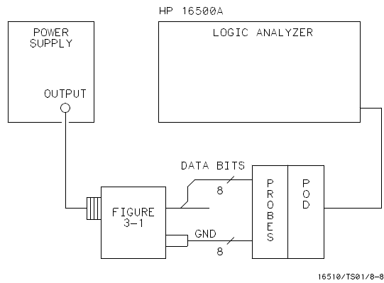
Figure 3-39. Equipment Setup For Threshold Accuracy
