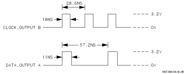
Figure 3-17. Pulse Generator Waveform For Test 3
