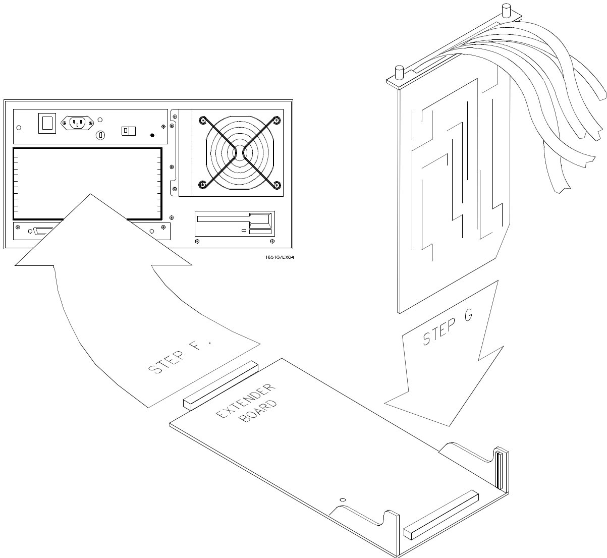
Figure 4-2. Extender Board And Module
