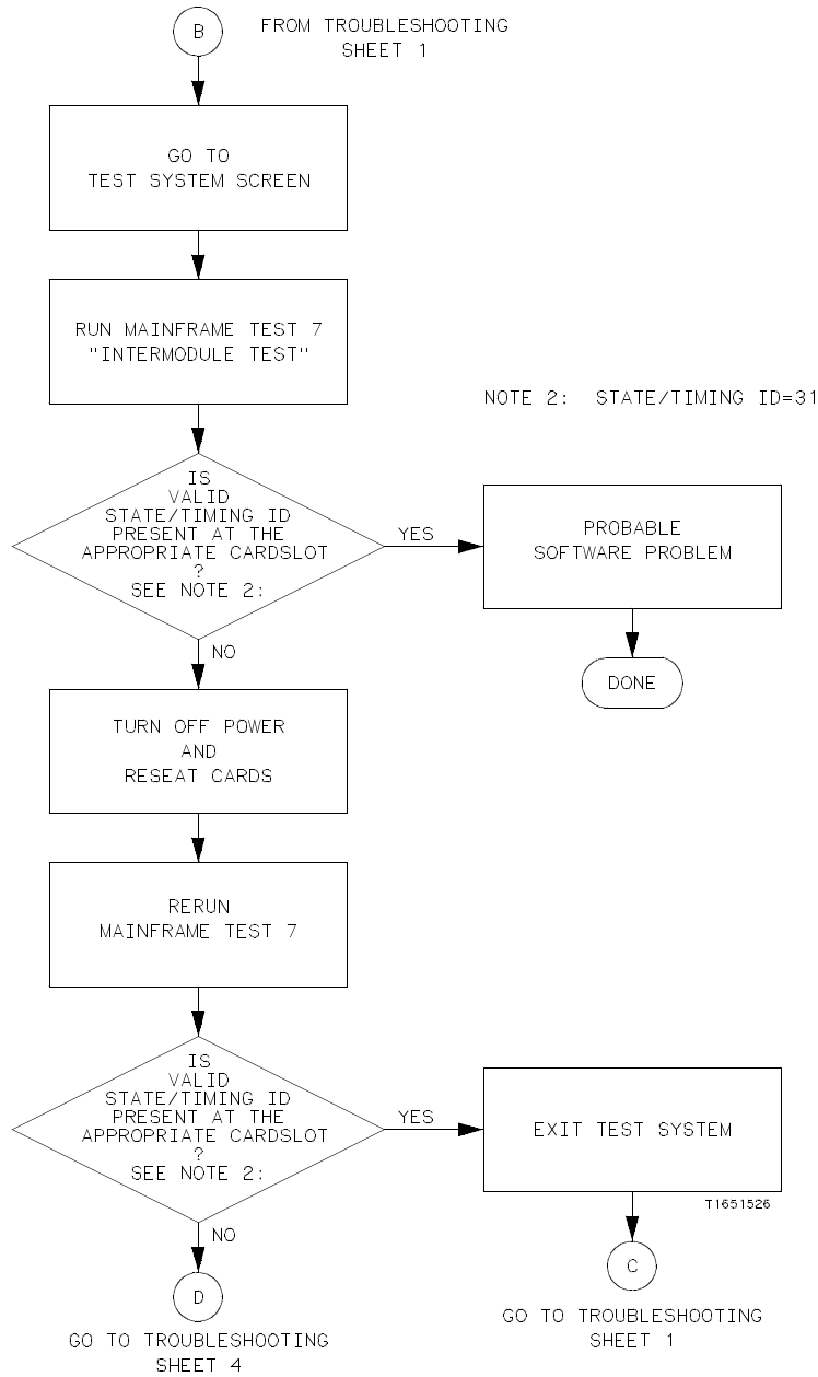
Figure 6-10. Troubleshooting Flowchart
