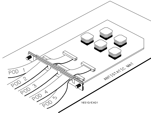
Figure 2-2. Cable Position
