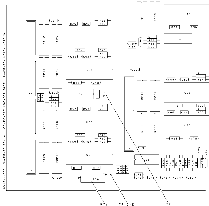
Figure 4-3. Adjustment Pod Location
