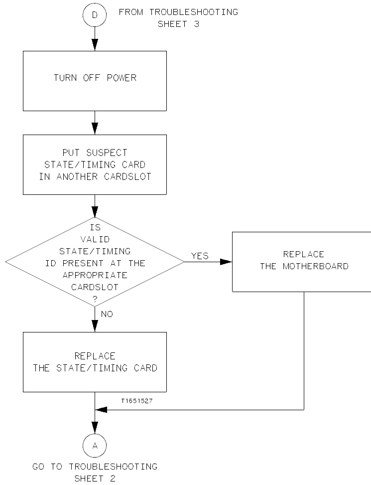
Figure 6-10. Troubleshooting Flowchart
