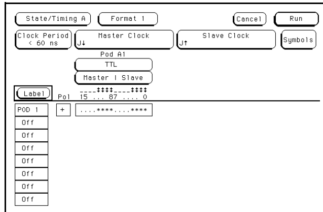
Figure 3-27. Format Screen
