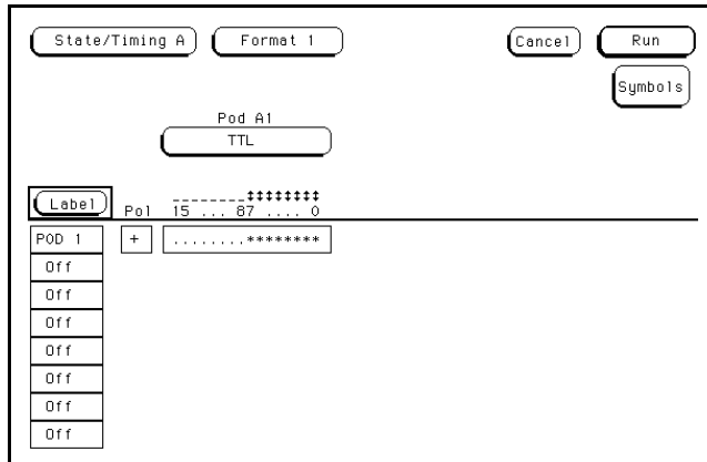
Figure 3-36. Format Screen
