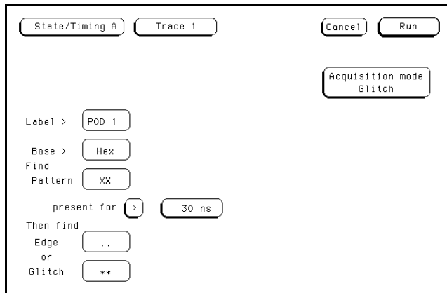
Figure 3-37. Trace Screen
