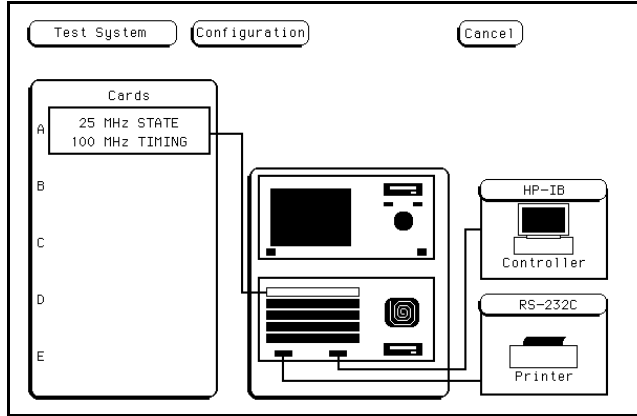
Figure 4-4. Startup Screen
