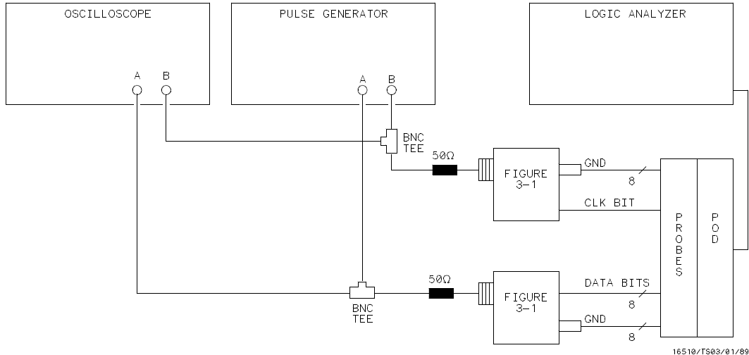
Figure 3-29. Equipment Setup For Test 7
