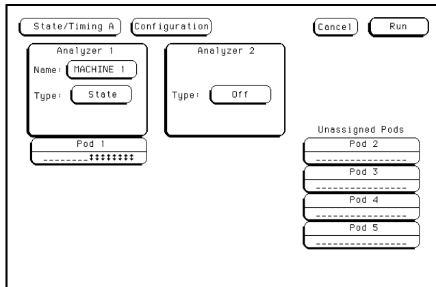
Figure 3-4. Configuration Screen
