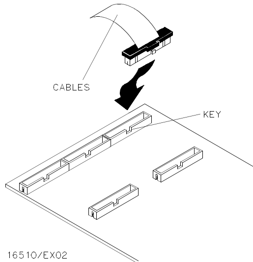
Figure 6-17. Card Connectors
