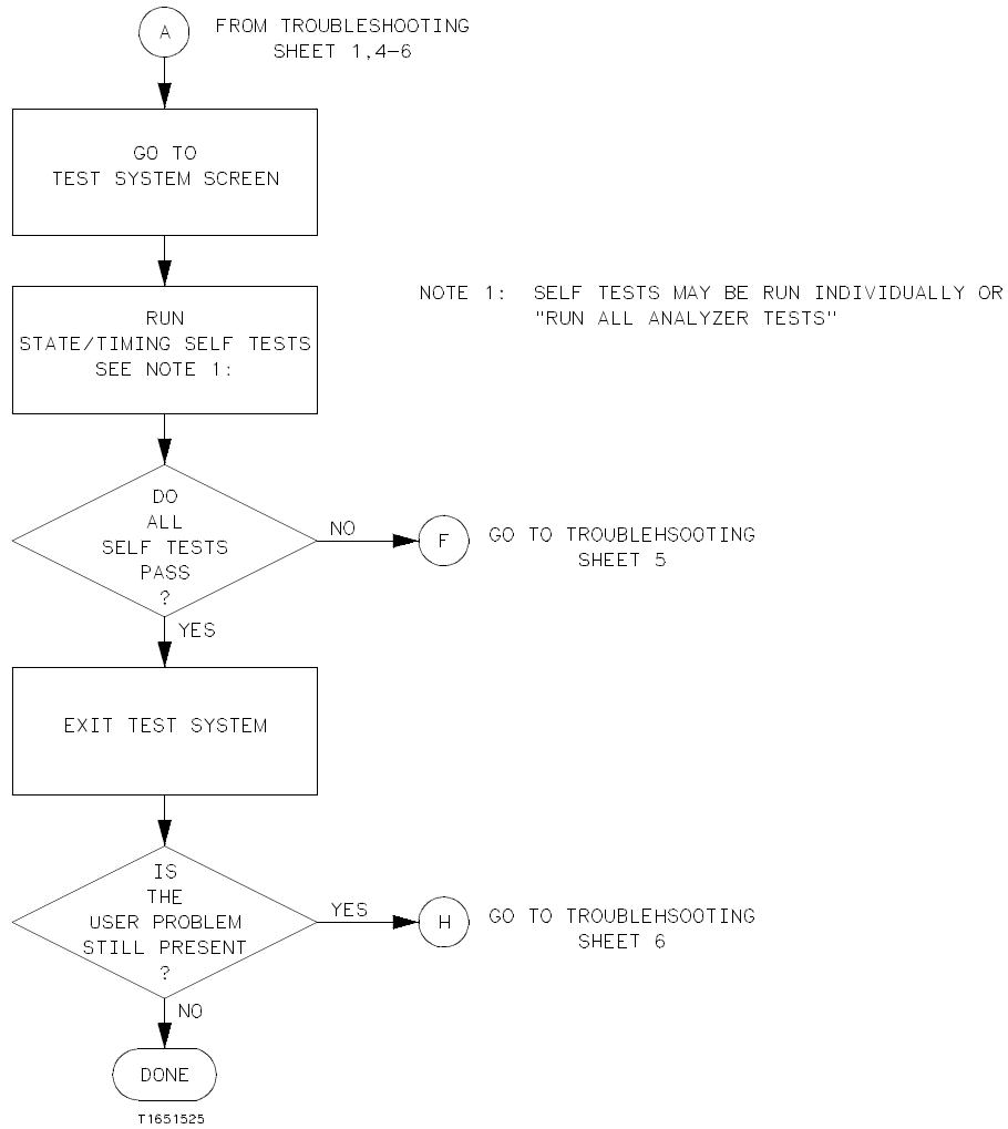
Figure 6-10. Troubleshooting Flowchart
