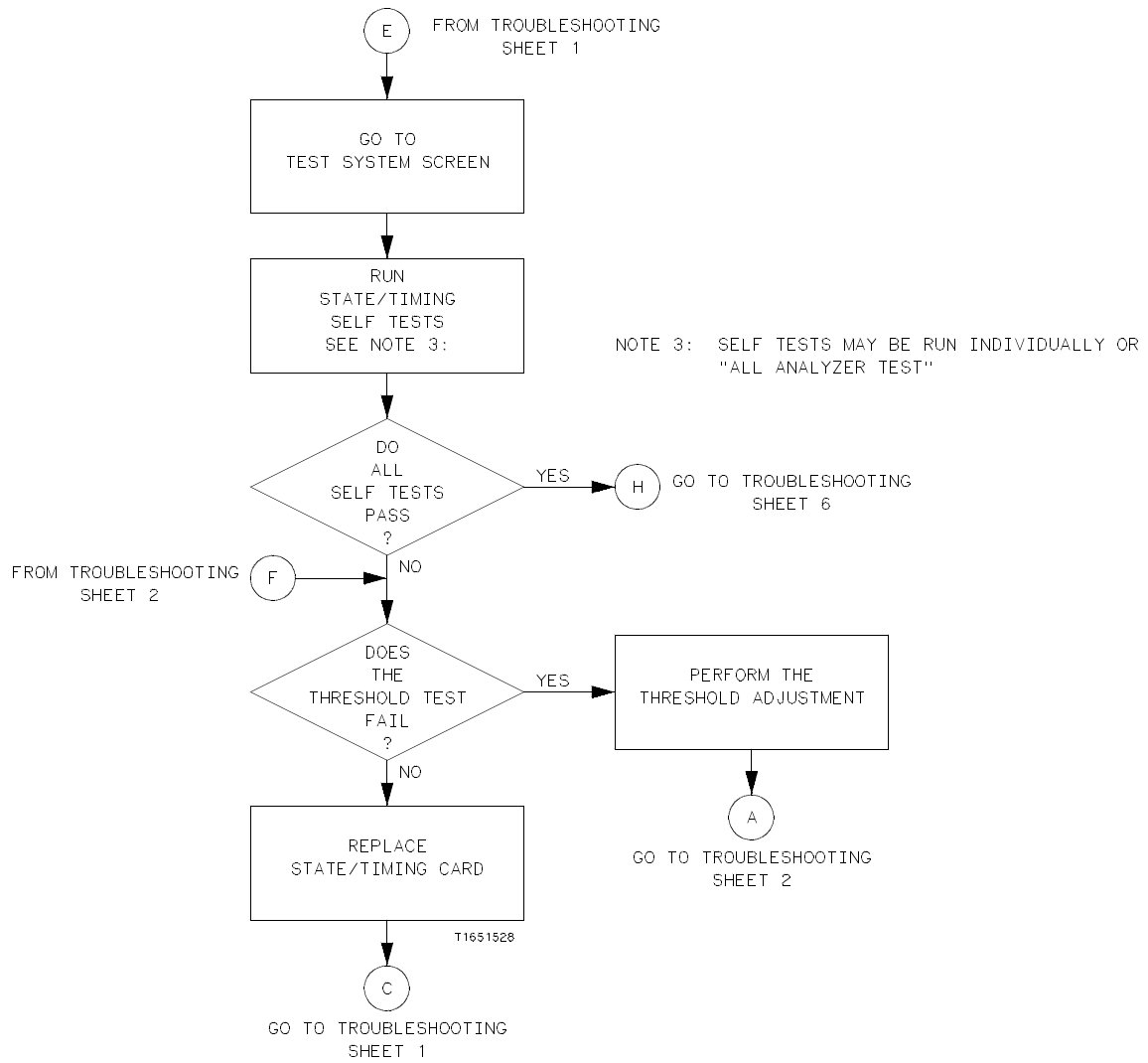
Figure 6-10. Troubleshooting Flowchart
